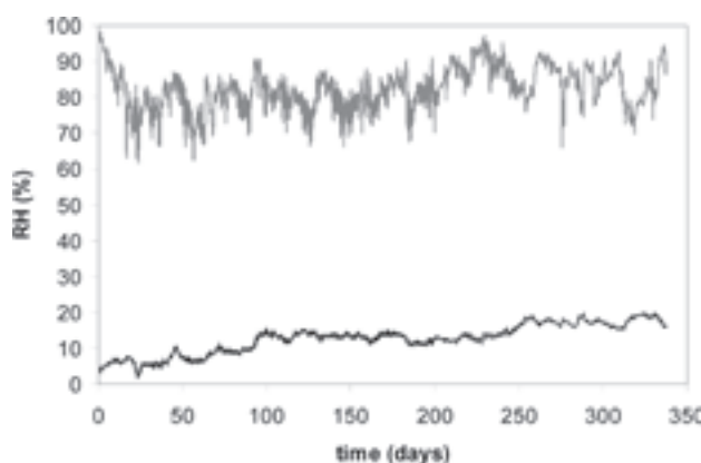
Fig. 2 Performance of low RH showcase, atmosphere below 20% is maintained for almost one year.
