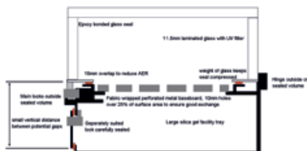
Fig. 1 Cross-section of design for low RH showcase with relevant features described.
