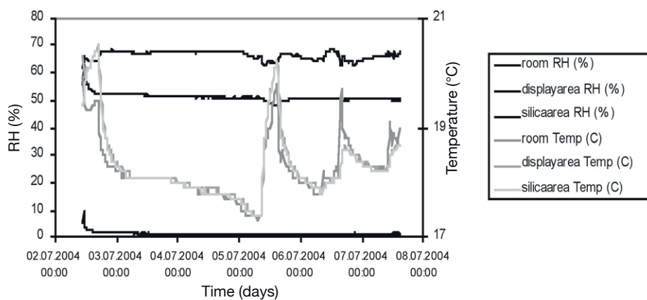
Figure 2: Conditions in various compartments of commercial case
