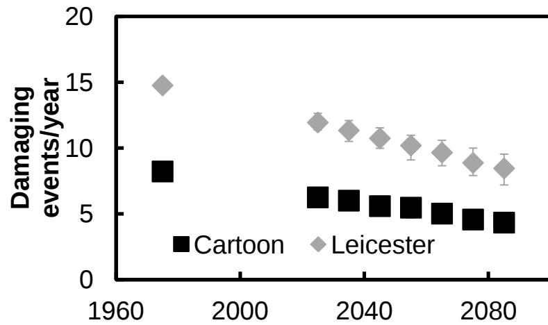
Figure D13: Impact of climate change on 20% humidity shocks.
