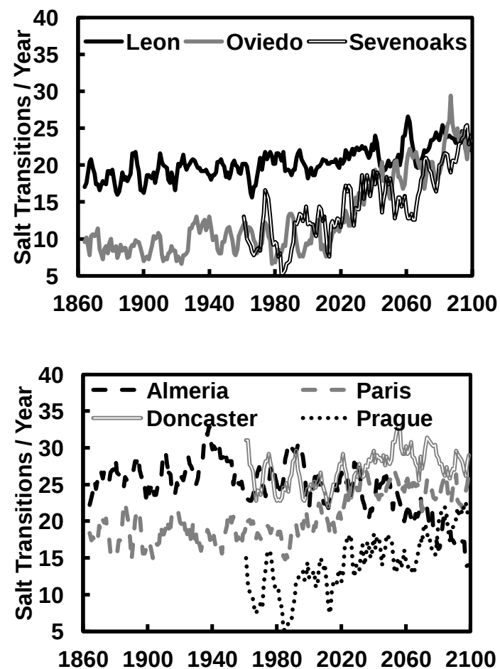
Figure C4 a and b: the impact of climate change on salt transitions at a critical humidity of 60%. Seven European locations are shown, with (a) having three of these and (b) the remaining four, these were split for clarity. Results are presented as five year smoothed averages from 1860 to 2100.
