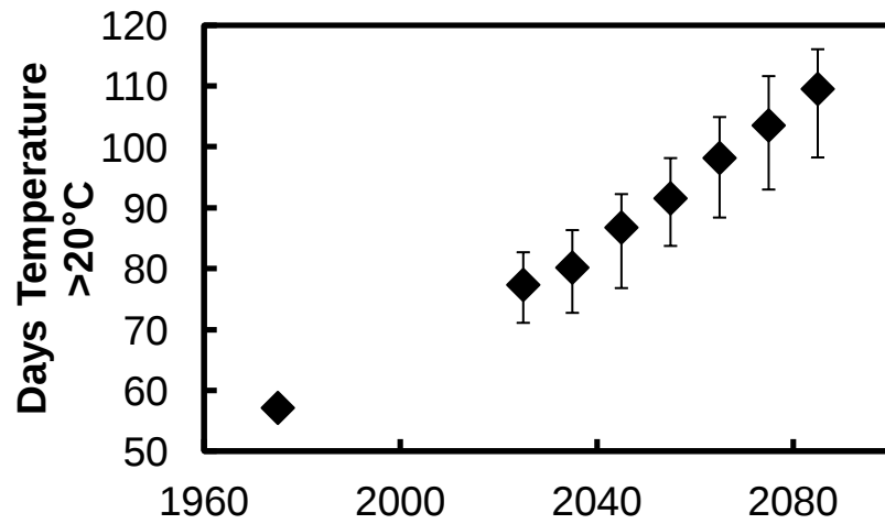
Figure D25: Impact of climate change on days temperature >20°C.
