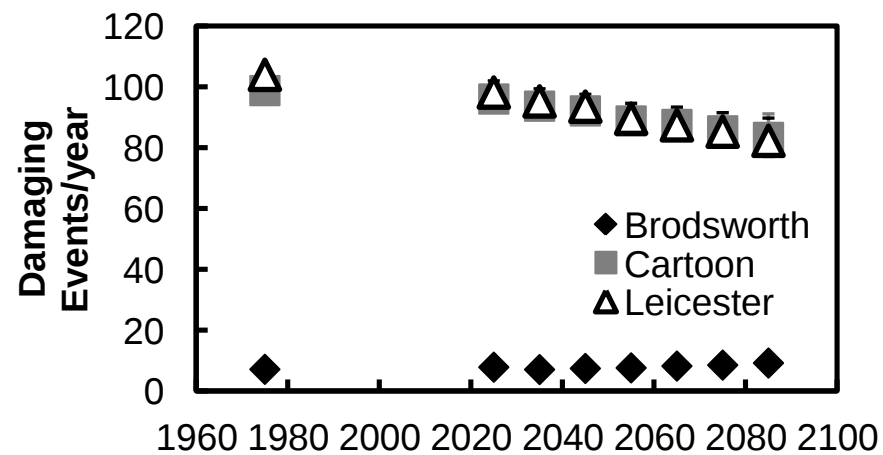
Figure D75: Impact of climate change on White Oak desorption events.
