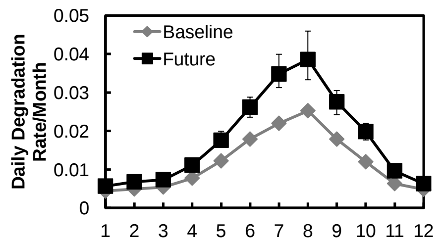
Figure D4: Seasonal impact on the Isoperm damage function.
