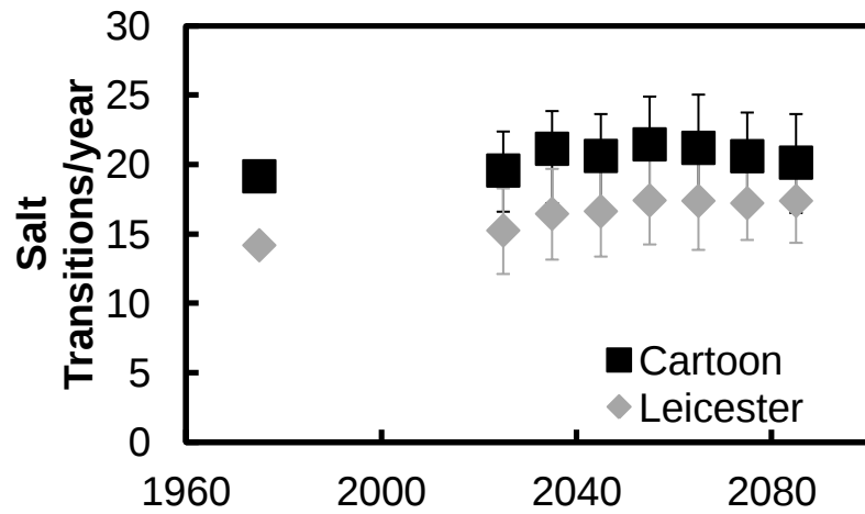
Figure D9: Impact of climate change on 60% salt transitions.
