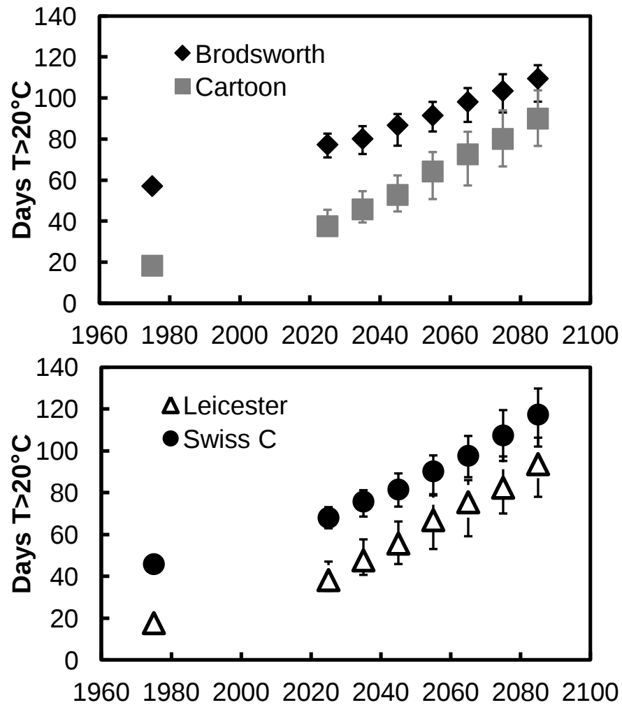
Figure D61 a and b: Impact of climate change on days where the temperature >20°C. Split here for clarity.
