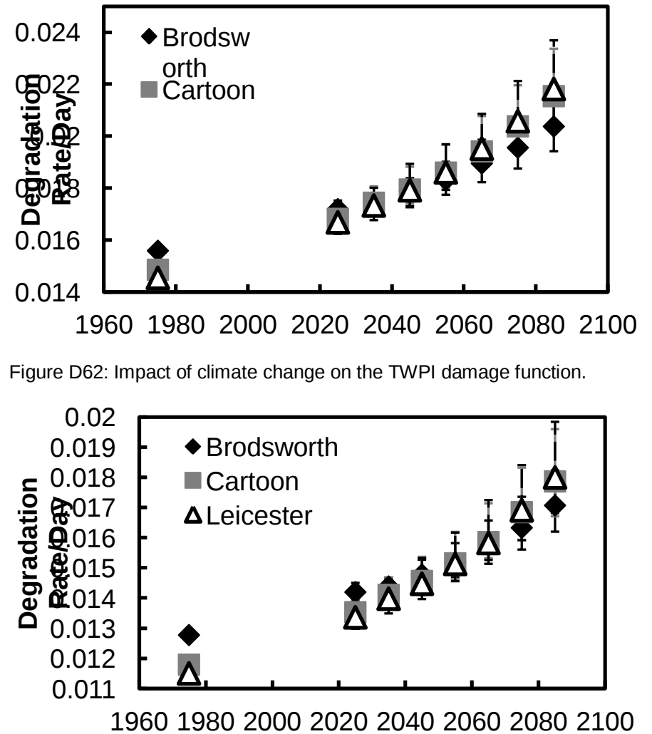
Figure D63: Impact of climate change on the isoperm damage function.
