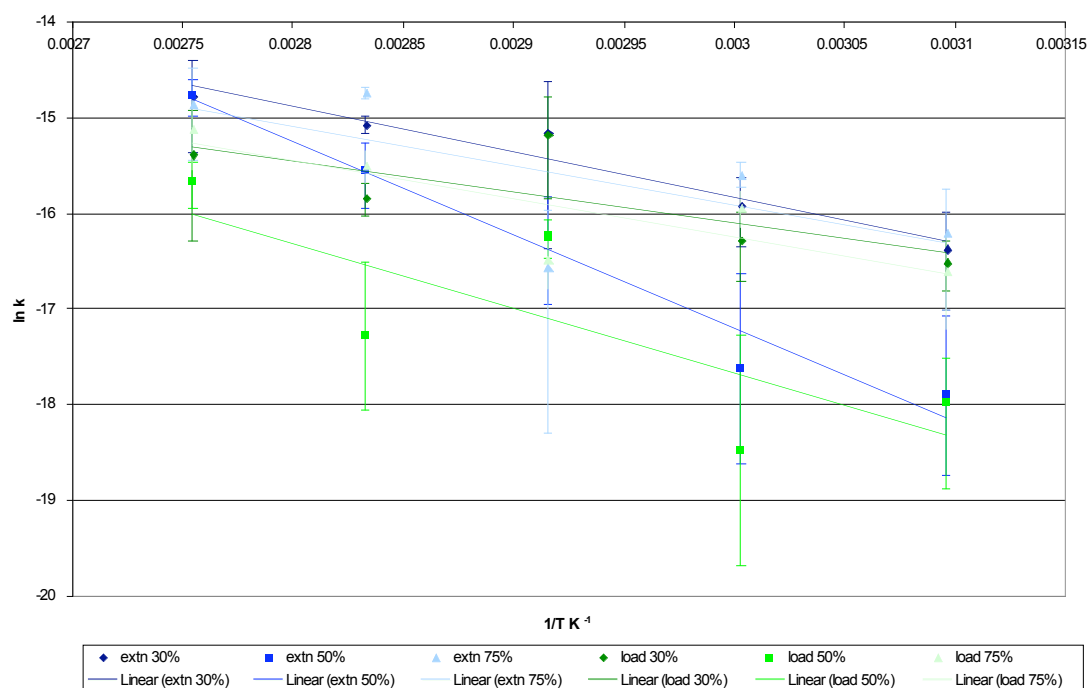
FIGURE 5. Arrhenius plot for tensile testing results
