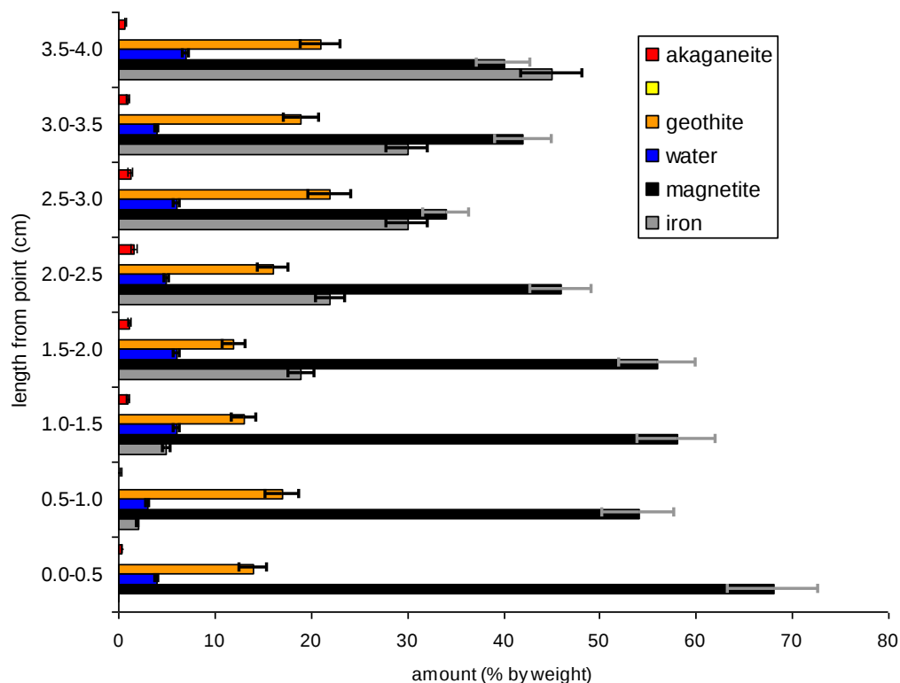
Figure 4.11 Analysis of species present in nail from Stonea by thermo-magenometry.
