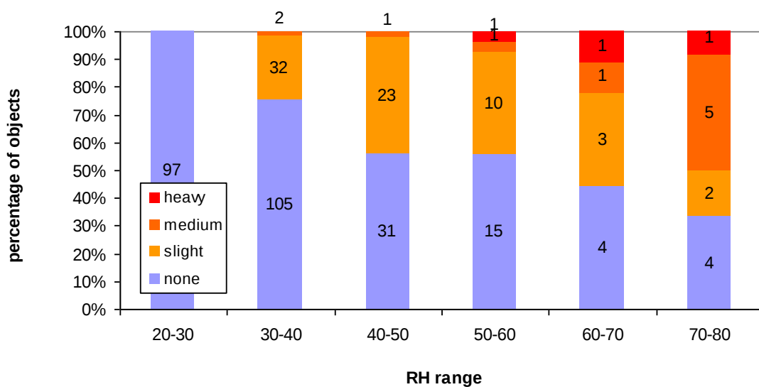
Figure 5.21 Normalised assessment of condition of archaeological iron objects in showcases with different maximum relative humidities and low ethanoic acid concentrations (no wood products present).
