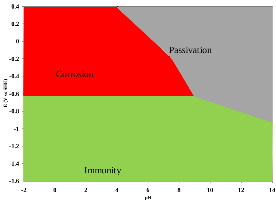
Figure 1.4 pH-Eh diagram for the system iron-water at 25°C showing different thermodynamic areas of stability (after Pourbaix, 1977).
