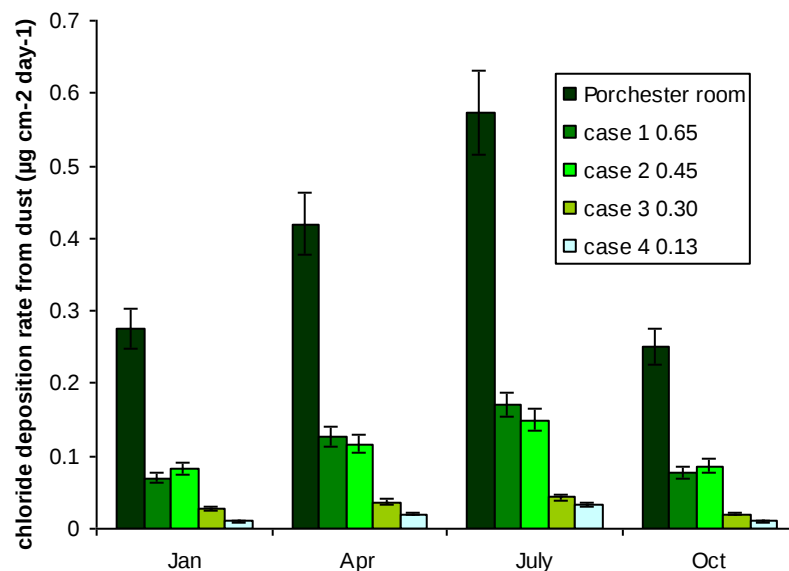
Figure 7.29 Chloride deposition as dust inside trial showcases at Portchester Castle
