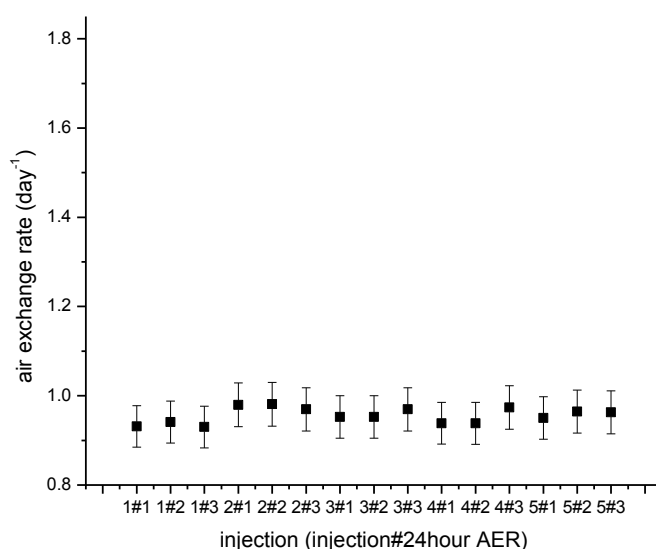
Figure 3.12 Repeat air exchange measurements without opening door.
