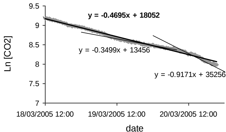
Figure 3.10 Differences in air exchange rate resulting from using short time periods.
