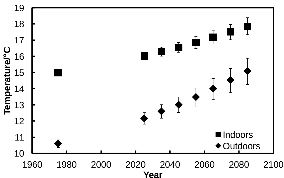
Figure 6.58: The annual average projected temperature in the Swiss Cottage. Error bars represent the interquartile range.
