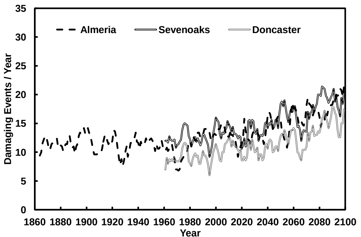
Figure 5.18 a and b: The projected impact of climate change on the number of damaging events indoors to cotton wood, caused by desorption of moisture. (a) presents four of seven European locations and (b) the remaining three. Results are plotted as five year smoothed averages. The baseline period medians of all locations are significantly different to those of the corresponding far future period.
