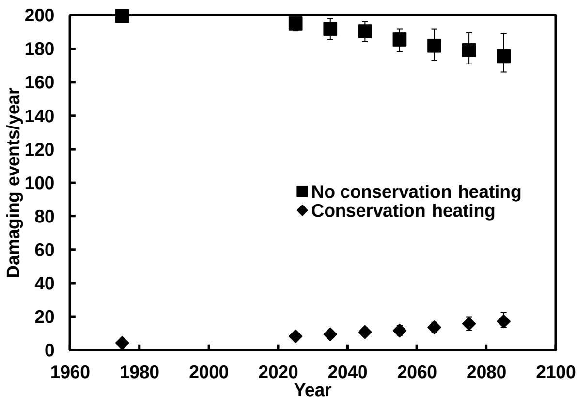
Figure 7.4: The impact of climate change on the application of conservation heating, with respect to the total number of damaging events to white oak, resulting from both adsorption and desorption events. Error bars represent the interquartile range.
