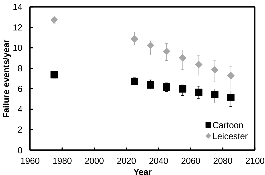
Figure 6.36: The annual average projected number of failure events in the Cartoon and Leicester Galleries at Knole. Error bars represent the interquartile range.
