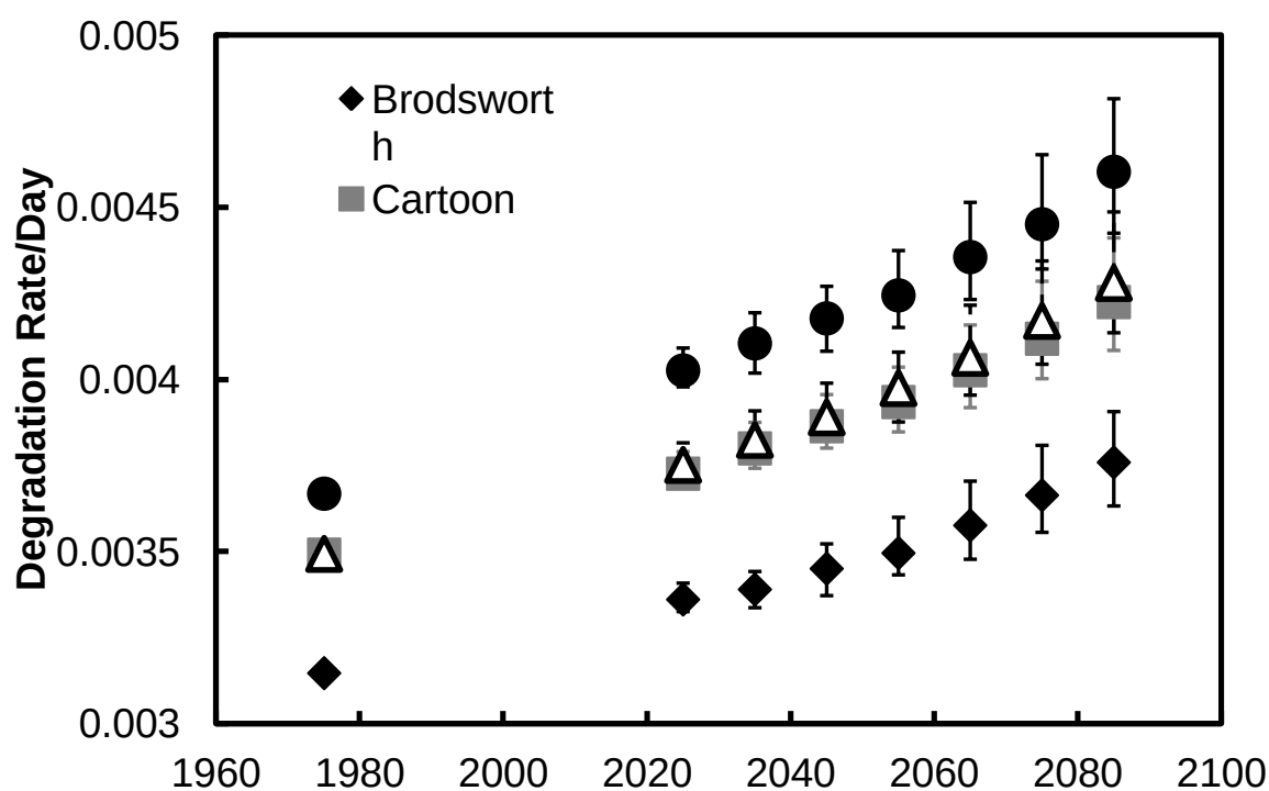
Figure 6.72: The annual average projected silk chemical degradation rate across all locations. Error bars represent the interquartile range.
