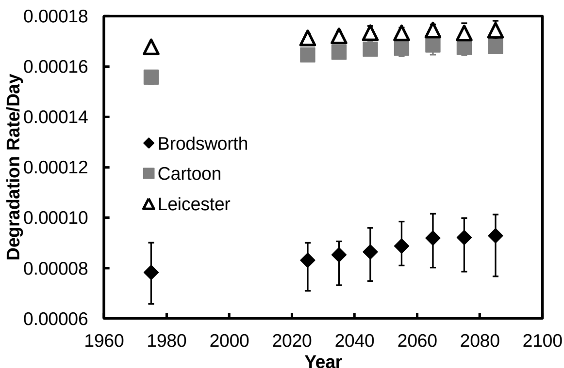
Figure 6.71: The annual average projected chemical degradation rate of paper across all locations, using the Pretzel function. Error bars represent the interquartile range.
