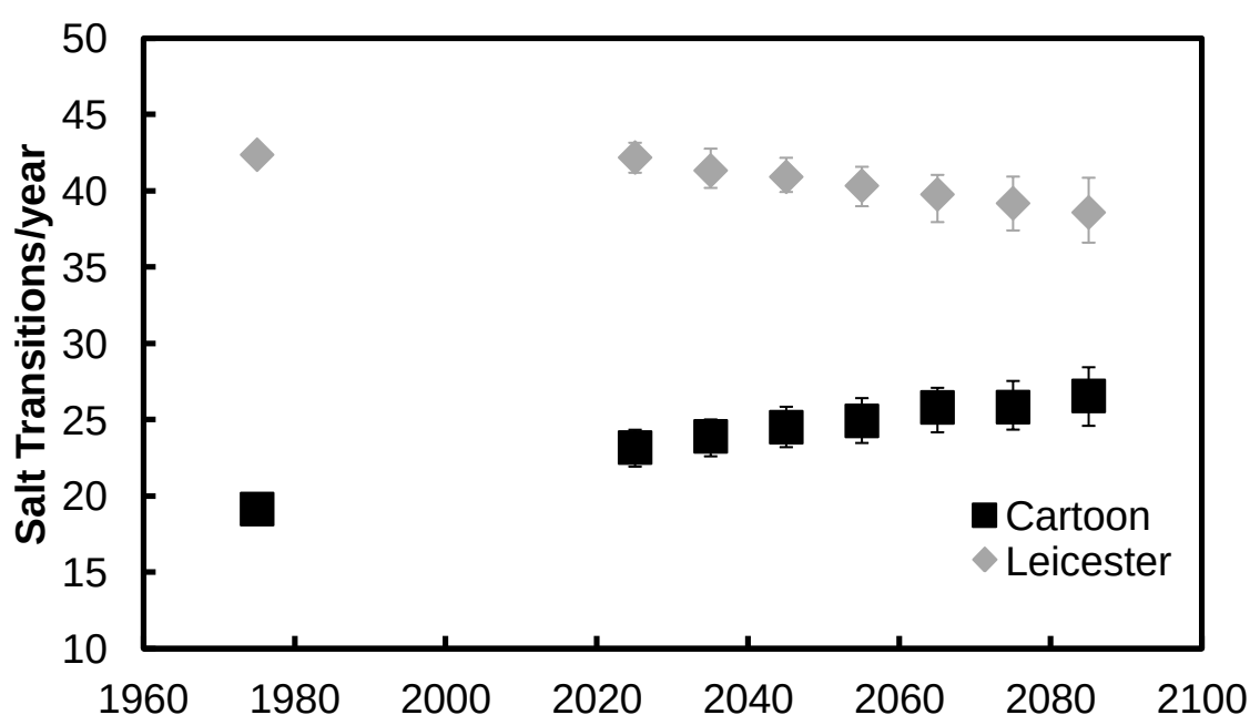
Figure 6.24: The annual average projected number of 85% salt transitions in the Cartoon and Leicester Galleries at Knole. Error bars represent the interquartile range.
