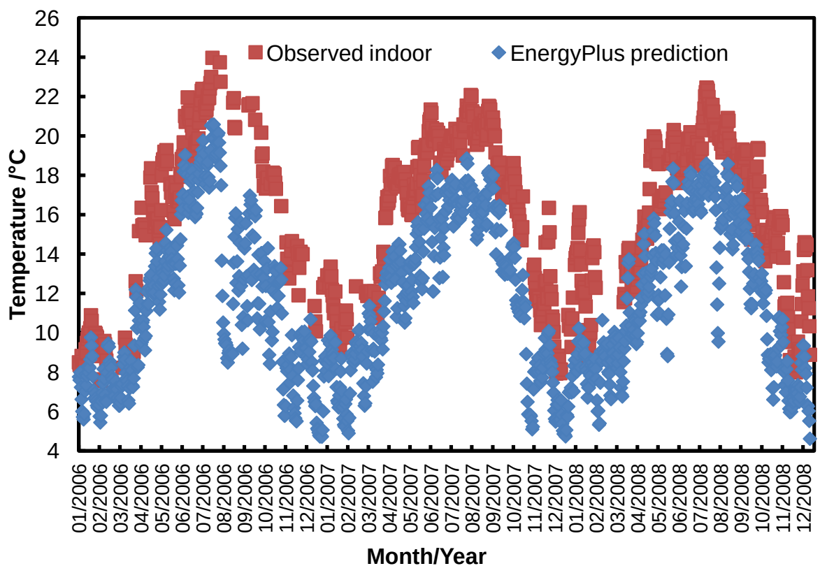
Figure 3.29: Predicted indoor temperature from EnergyPlus, compared to the observed temperature in the Library at Brodsworth Hall over the period 01/2006-12/2008.
