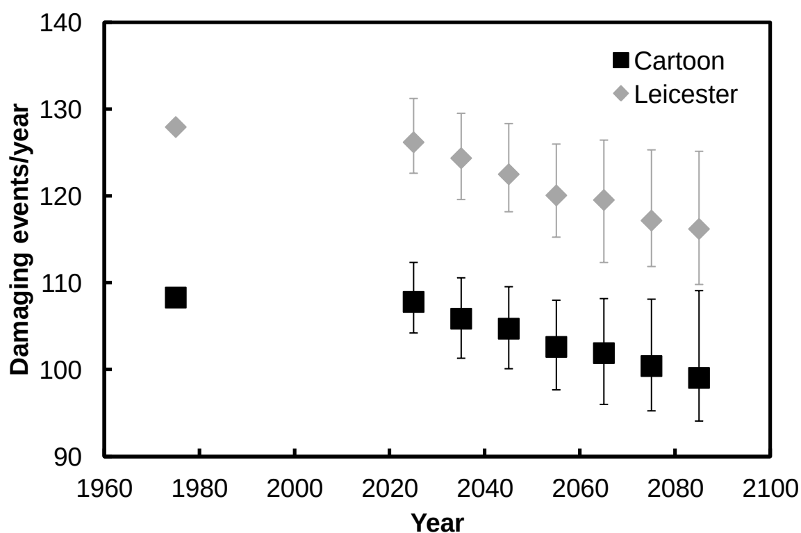
Figure 6.32: The annual average projected number of damaging events arising from adsorption of moisture in the Cartoon and Leicester Galleries at Knole. Error bars represent the interquartile range.
