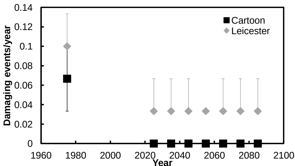
Figure 6.30: The annual average projected number of damaging events arising from a 40% humidity change in the Cartoon and Leicester Galleries at Knole. Error bars represent the interquartile range.
