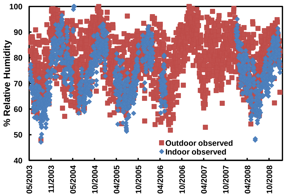
Figure 2.10: Observed indoor relative humidity in the Leicester Gallery at Knode over the period 06/2003-12/2008. Observed outdoor relative humidity for Gatwick.
