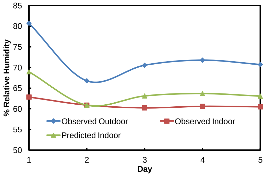
Figure 3.52: Comparison of the observed relative humidity indoors and outdoors to the indoor relative humidity forecast for the Cartoon Gallery at Knole.
