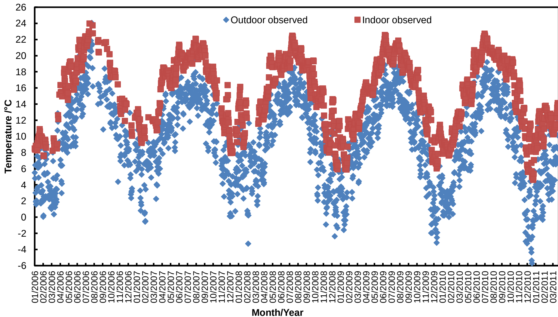
Figure 3.1: Daily average temperature indoors in the Library and outdoors at Brodsworth Hall for the period 01/2006-03/2011.
