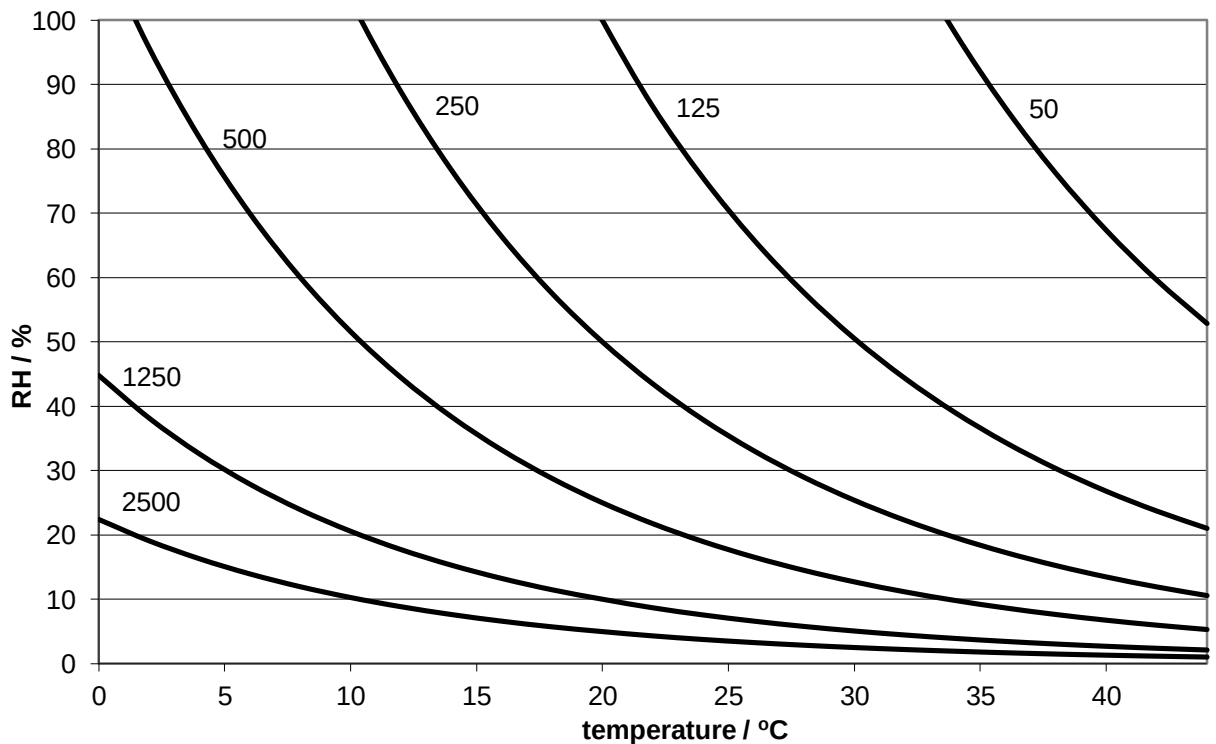
Figure 4.3: Isotherms for silk deterioration (predicted display lifetimes in years, are shown next to each isotherm). Reproduced from Luxford (2009).
