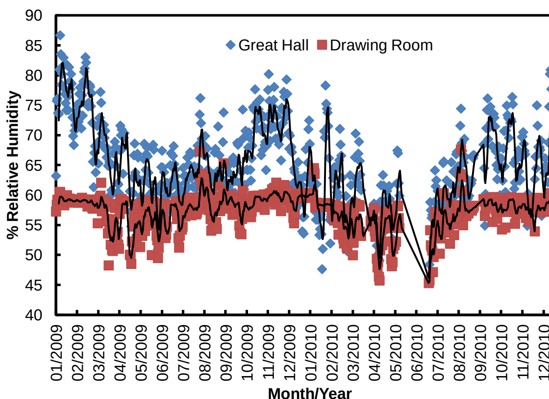
Figure 3.39: Comparison of the relative humidity in the unheated Great Hall and the controlled Drawing Room at Canons Ashby, for the period 01/2009-12/2010. The five day moving average is also plotted over the daily averages.
