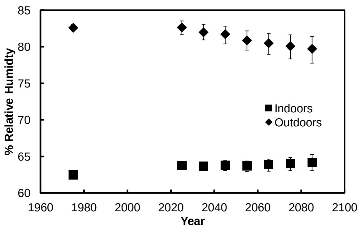
Figure 6.59: The annual average projected % relative humidity in the Swiss Cottage. Error bars represent the interquartile range.
