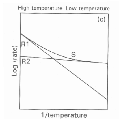
Figure 4.1: Reproduced from Brimblecombe (1994), highlighting the nonlinearity in the summation of two Arrhenius plots.
