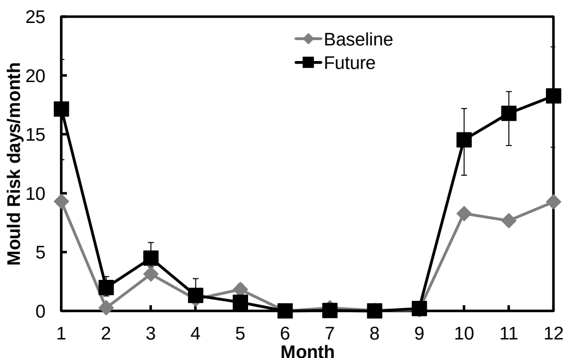
Figure 6.17: The monthly average projected number of mould risk days derived from the critical relative humidity damage function in the Cartoon and Leicester Galleries at Knole. Error bars represent the interquartile range.
