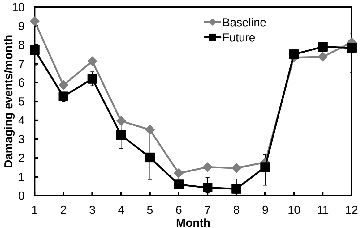
Figure 6.35: The monthly average projected number of damaging events arising from desorption of moisture in the Cartoon Gallery at Knoke. Error bars represent the interquartile range.
