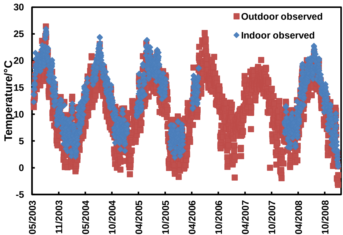
Figure 2.9: Observed indoor temperature in the Leicester Gallery at Knode over the period 06/2003-12/2008. Observed outdoor temperature for Gatwick.
