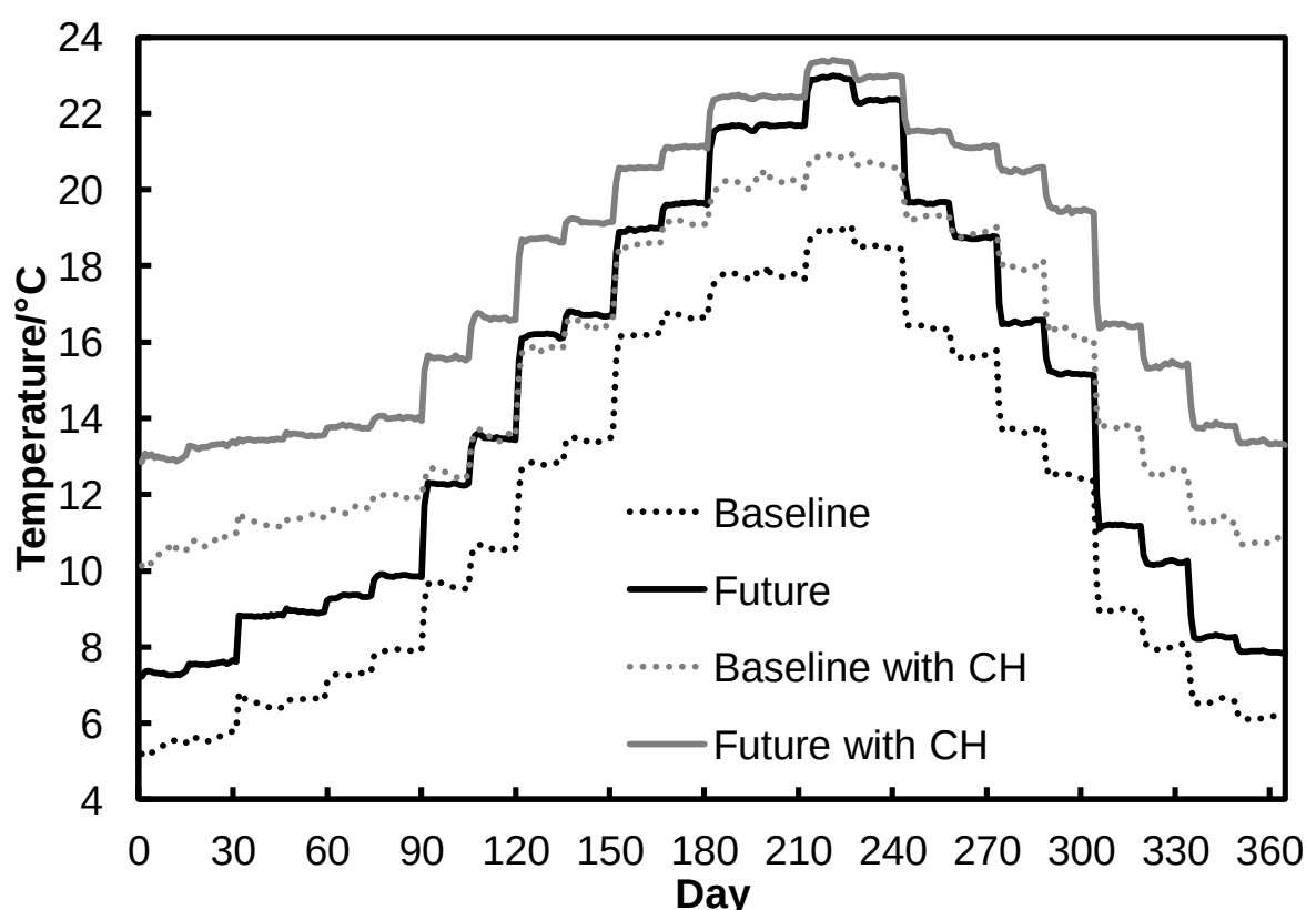
Figure 7.1: The impact of climate change on the application of conservation heating in the Cartoon Gallery at Knole. Each line represents the median value, which is presented for each day across the year, from the 100 runs of the weather generator.
