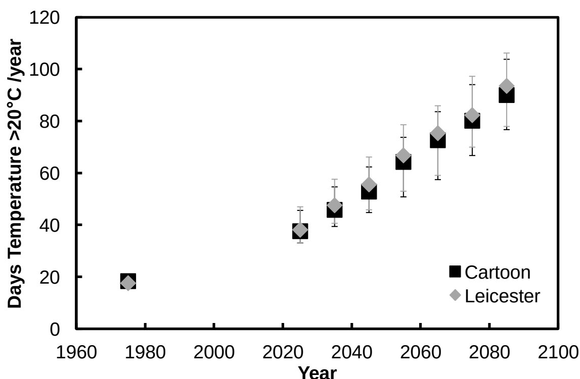
Figure 6.6: The number of days projected per year with an average temperature exceeding 20°C in the Cartoon and Leicester Galleries at Knole. Error bars represent the interquartile range.
