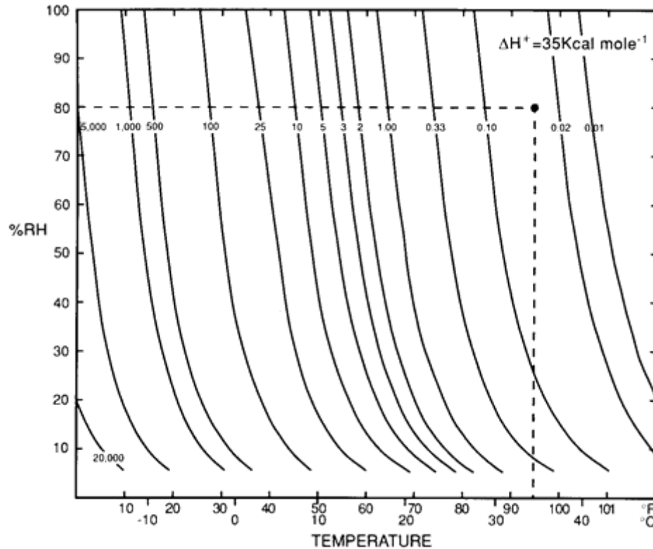
Figure 4.2: Reproduced from Sebera (1994). Percent relative humidity versus temperature Isoperm diagram. Permanence values are calculated for \Delta H = 35 kcal relative to paper at 68 degrees F and 50% RH taken as comparison standard (permanence equal to 1.00). Relative permanence at 95 degrees F and 80% RH is 0.03.
