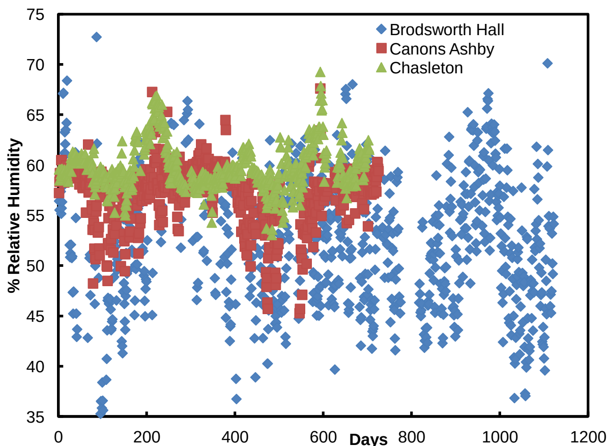
Figure 3.35: Comparison of the relative humidity in three rooms with conservation heating at Brodsworth Hall, Canons Ashby and Chasleton. The data at Brodsworth Hall covers three years, and the other two locations two years. Each location covers a different time period; however they all begin at the start of January.
