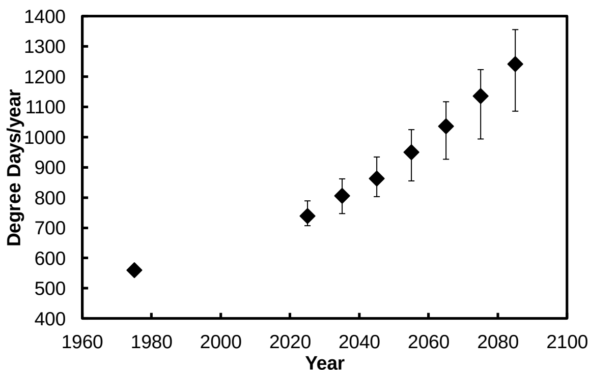
Figure 6.66: The annual average projected number of degree days in the Swiss Cottage. Error bars represent the interquartile range.
